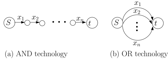
Fig. 2. AND and OR technologies. In AND (a), the project is successful if a packet is routed along a linear path (where each agent controls an edge), and in OR (b), the project is successful if a packet is routed at least along one edge.
