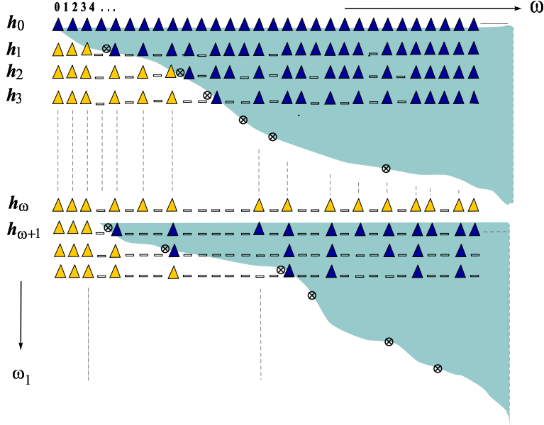
Figure 3.2: THE INDUCTIVE CONSTRUCTION. Illustration of an initial segment of the sequence \langle h_\alpha \mid \alpha < \omega_1 \rangle up to h_{\omega_2} . For each bad sequence h_\alpha , the bright trees are the fixed (limit) trees taken from the previous bad sequence, while the dark ones are those in Dg_\alpha . The shaded background represents the domains Dg_\alpha . At the limits, these domains vanish, and the limit sequences contain only the limit trees. Note that a fixed tree in h_n for n \in \mathbb{N} is fixed only up to \omega , after which it can be reduced again by some of its proper subtrees. This rule applies to all limits less than \omega_1 .
